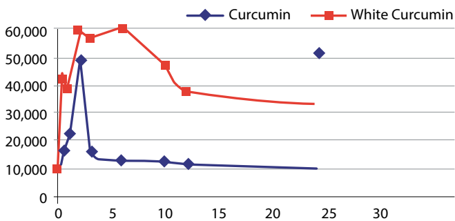
Absorption of curcumin (600mg/Kg) and CuroWhite (25mg/Kg) in blood plasma
